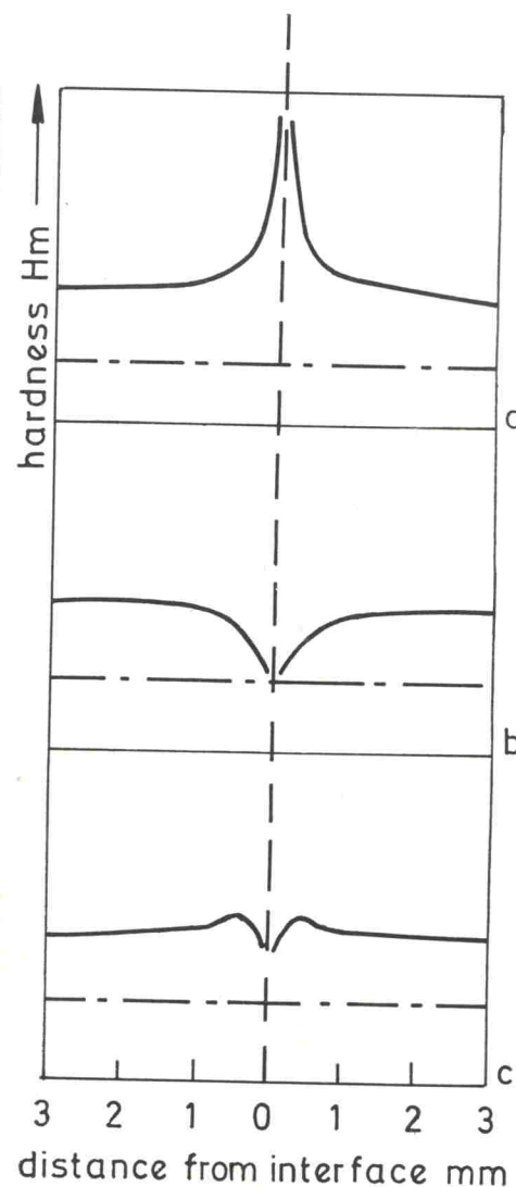
52 Typical hardness profiles observed when two similar metals are welded under different welding conditions.
