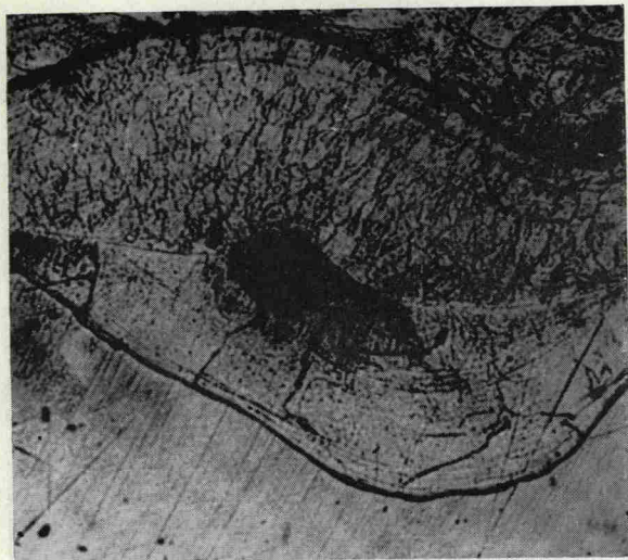
53 Solidification cavity in copper-to-nickel bond. \times 280 . [Courtesy Weld. Research Council. (Holtzman and Cowan. 21 )
